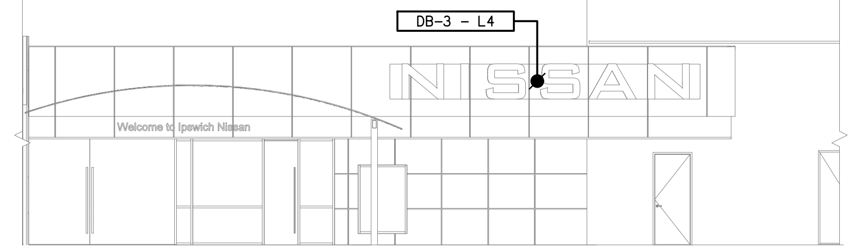
NISSAN SOUTH EXTERNAL BUILDING ELEVATION SCALE 1:100
