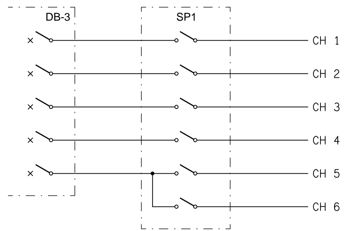
SCHEMATIC SP1 LIGHTING CONTROL NOT TO SCALE
